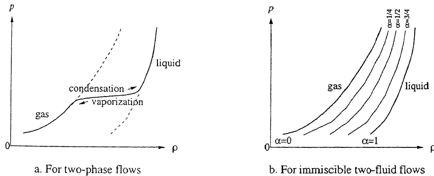
FIG. 1. Pressure-density diagrams.
